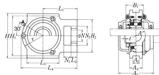
Cast dust cover type Open end C-UKT...D1 Closed end CM-UKT...D1
