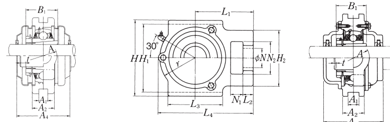
Cast dust cover type
