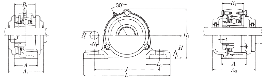
Cast dust cover type Open end C-UKP...D1 Closed end CM-UKP...D1
