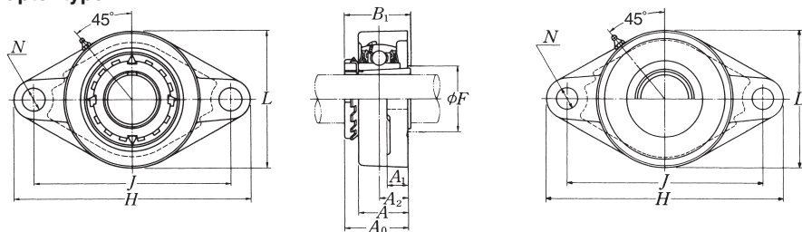
Pressed steel dust cover type
