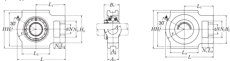
Pressed steel dust cover type
