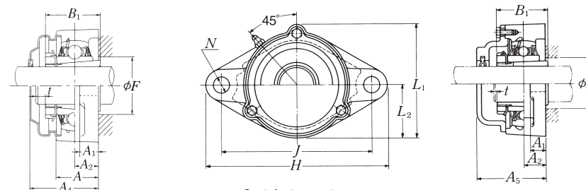
Cast dust cover type
