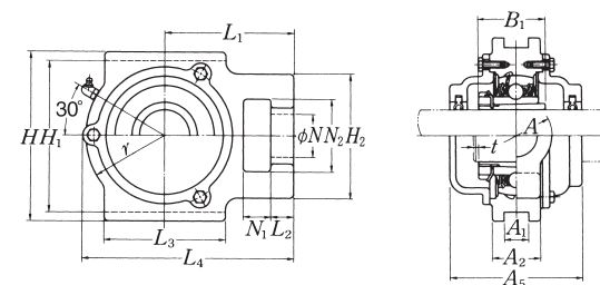
Cast dust cover type
