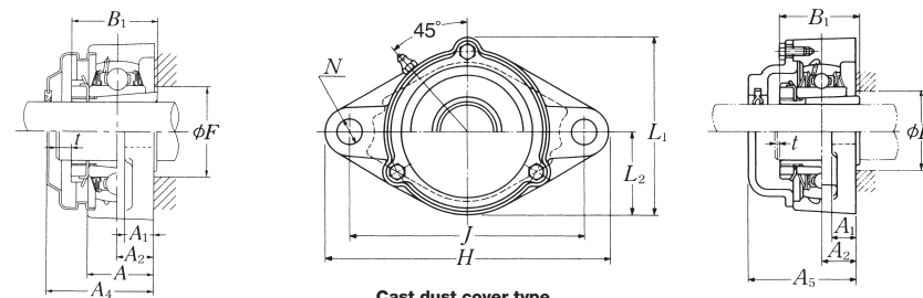
Cast dust cover type Open end C-UKFL...D1 Closed end CM-UKFL...D1
