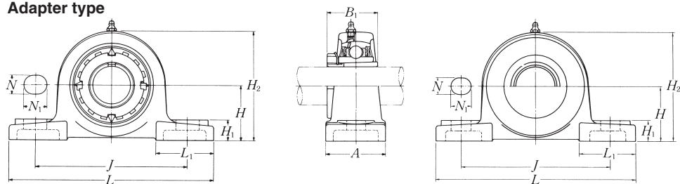
Pressed steel dust cover type Open end Z-UKP...D1 Closed end ZM-UKP...D1
