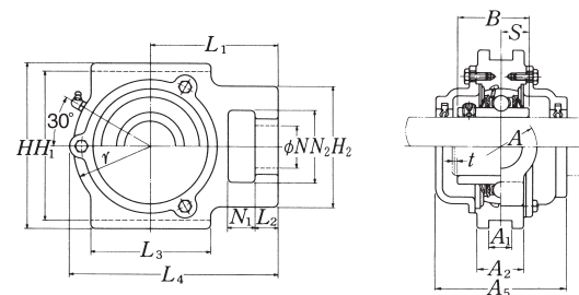
Cast dust cover type Open end C-UCT...D1 Closed end CM-UCT...D1
