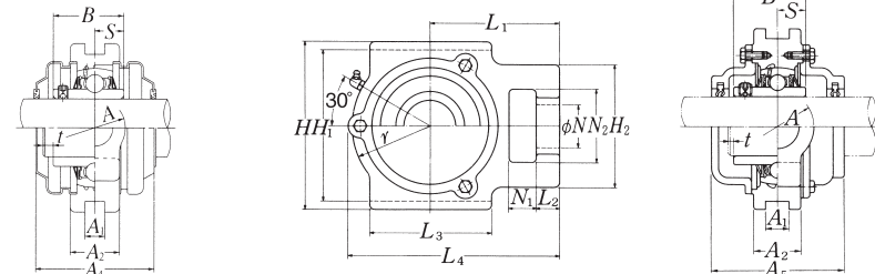
Cast dust cover type Open end C-UCT...D1 Closed end CM-UCT...D1
