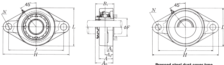
Pressed steel dust cover type Open end Z-UKFL...D1 Closed end ZM-UKFL...D1
