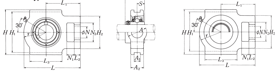
Pressed steel dust cover type Open end Z-UCT...D1 Closed end ZM-UCT...D1
