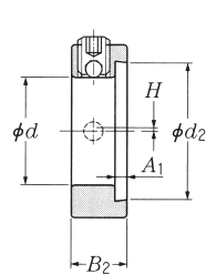
Eccentric locking collar
