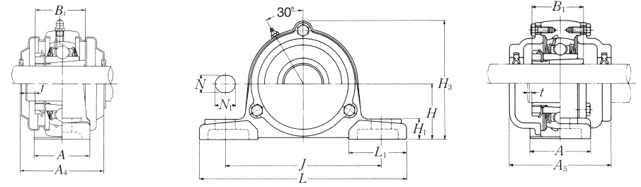
Cast dust cover type Open end C-UKP...D1 Closed end CM-UKP...D1
